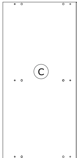
CA04203 720x353x16mm
