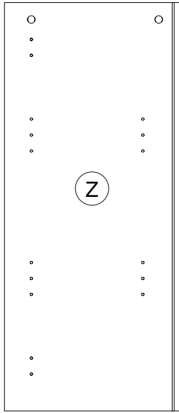
FI10011 820x352x16mm
